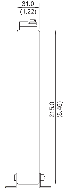
SIDE
